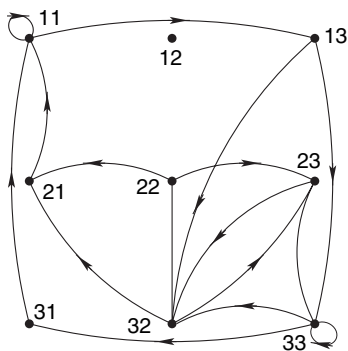
Figure 4.8 The digraph for Example 4.7.7.
