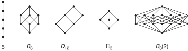
Figure 3.2 Some examples of posets.
