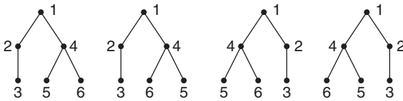
Figure A.2 Four plane trees.
