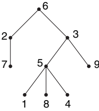
Figure A.1 A tree.
