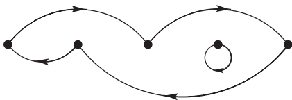
Figure 4.15 A representation of the permutation 31542.
