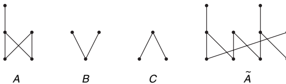
Figure 3.70 A solution to Exercise 3.10(c).
