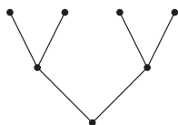
Figure 3.77 The complete dual binary tree P_3 .
