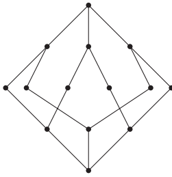
Figure 3.90 An interval in a putative “Fibonacci binomial poset”.
