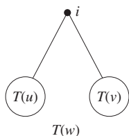
Figure 1.7 The definition of T(w) .
