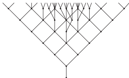
Figure 3.41 The Fibonacci differential poset Z_1 .
