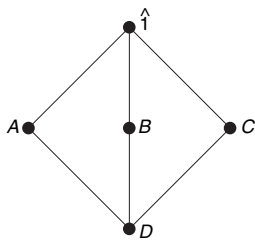
Figure 3.14 The poset related to equation (3.1).
