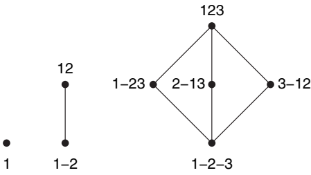
Figure 3.20 Small partition lattices.
