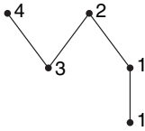
Figure 3.81 The poset P_{11324} when 13 = 31 , 14 = 41 , 24 = 42 .
