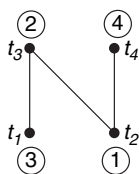
Figure 3.29 A labeled poset.
