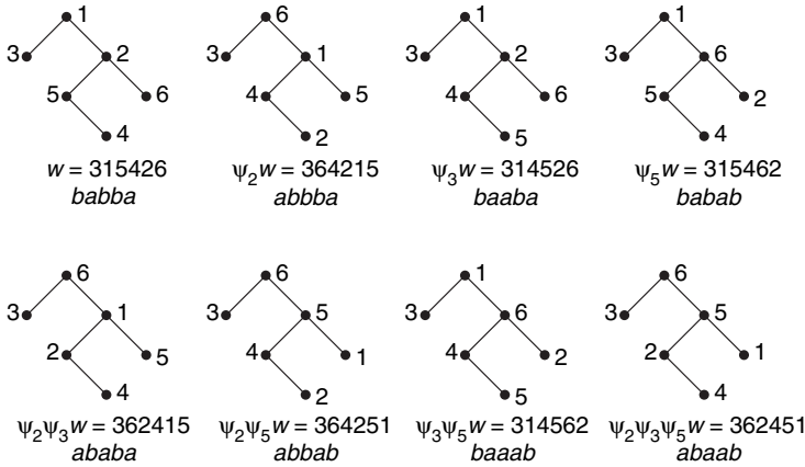
Figure 1.12 The M -equivalence class [315426] .
