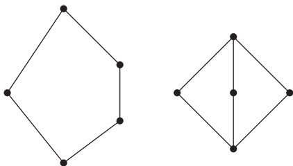
Figure 3.43 Obstructions to distributivity and modularity.
