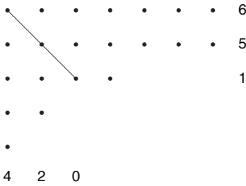
Figure 1.33 Frobenius notation.
