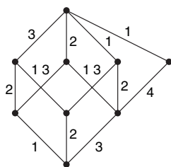
Figure 3.28 A nonlattice with an R-labeling.
