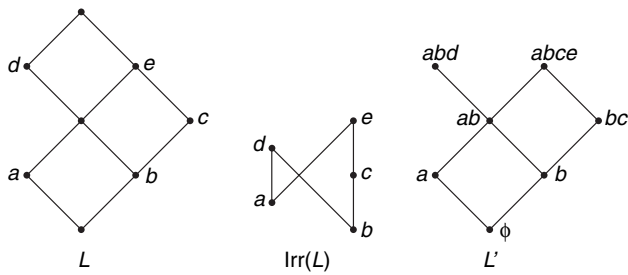
Figure 3.72 The MacNeille completion of \text{Irr}(L) .
