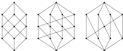
Figure 3.42 Which are lattices?
