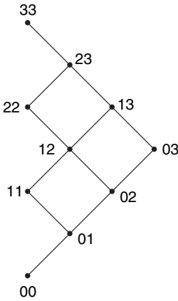
Figure 3.11 The distributive lattice J(2 \times 3) .
