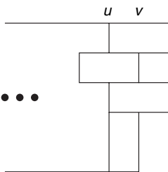
Figure 4.31 Dimers in columns u and v .
