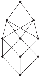
Figure 3.35 The join B_3 * B_2 .
