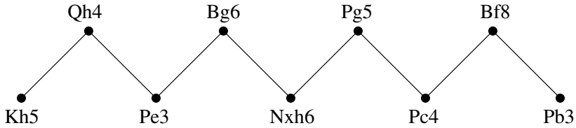
Figure 1.35 The solution poset for Exercise 1.145.
