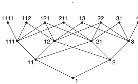
Figure 3.45 The composition poset \mathcal{C} .
