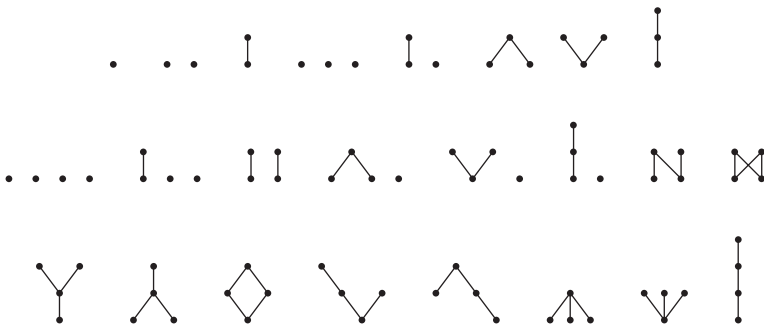
Figure 3.1 The posets with at most four elements.
