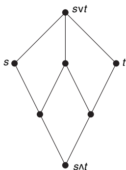
Figure 3.6 A semimodular but nonmodular lattice.
