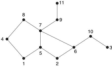
Figure 3.31 Nongraded posets satisfying the \delta -chain condition.
