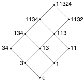
Figure 3.52 The distributive lattice L_{11324} when 13 = 31 , 14 = 41 , 24 = 42 .
