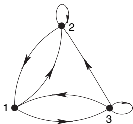
Figure 4.7 A digraph illustrating the transfer-matrix method.
