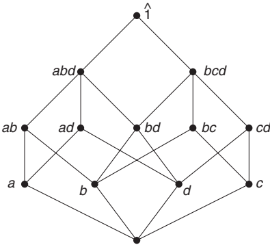
Figure 4.5 Face poset of the triangulation of Figure 4.4.
