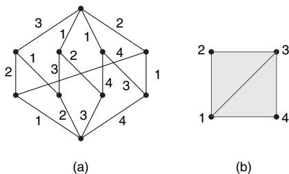
Figure 4.2 An edge-labeled face lattice and corresponding triangulation.
