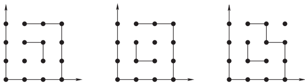
Figure 2.5 Three non-intersecting 2-paths.
