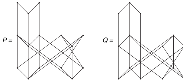
Figure 3.70 A solution to Exercise 3.10(c).
