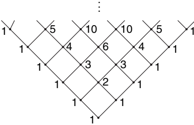
Figure 3.12 The distributive lattice J_f(\mathbb{N} + \mathbb{N}) .
