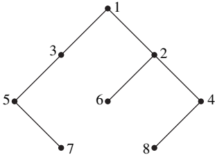
Figure 1.8 The increasing binary tree T(57316284) .
